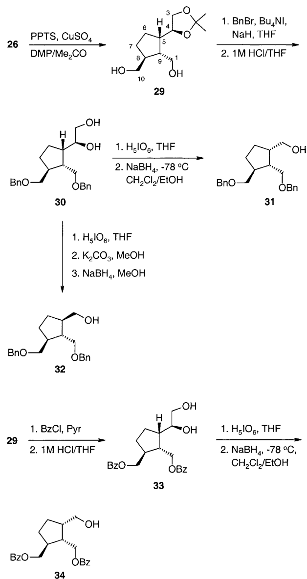
Scheme 3. Preparation of Building Blocks
